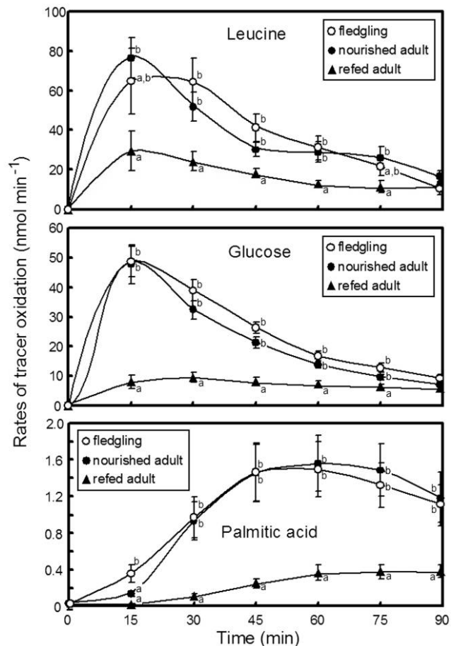
Figure 3. Instantaneous rates of exogenous tracer oxidation in fledgling, fed adult, and refed adult zebra finches. Different letters indicate significant differences between treatment groups at a given time according to ANOVA and Dunn's post hoc pairwise comparisons.
