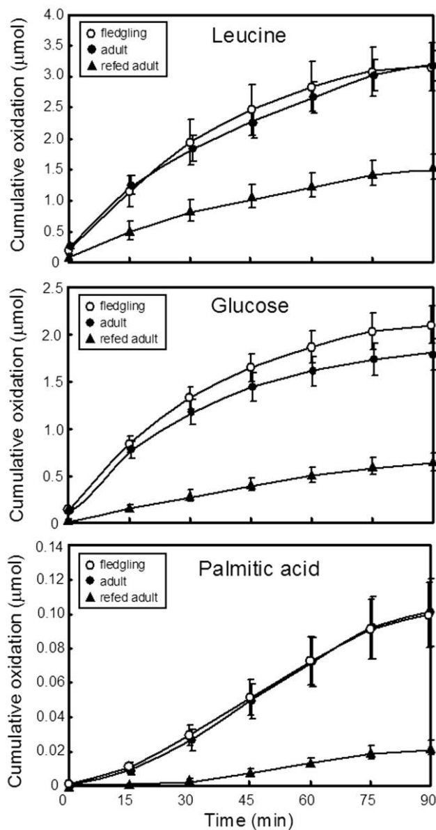
Figure 4. Cumulative rates of exogenous tracer oxidation in fledgling, fed adult, and refed adult zebra finches. Data points are slightly offset for clarity. See Table 3 for model parameters.
